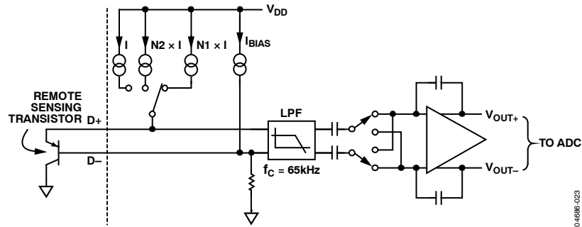
Figure 26. Signal Conditioning for Remote Diode Temperature Sensors
