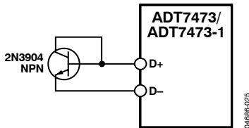
Figure 27. Measuring Temperature Using an NPN Transistor
