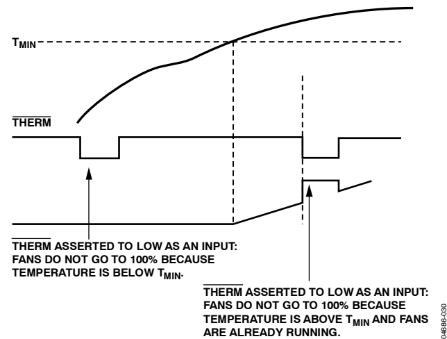
Figure 33. Asserting \overline{\text{THERM}} Low as an Input in Automatic Fan Speed Control Mode
